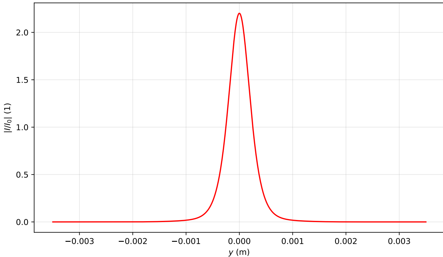
Intensity profile I(x=0, y, z=2.149)/I_0 , \text{Pin}=1.0\text{Pcr} , artificial time
